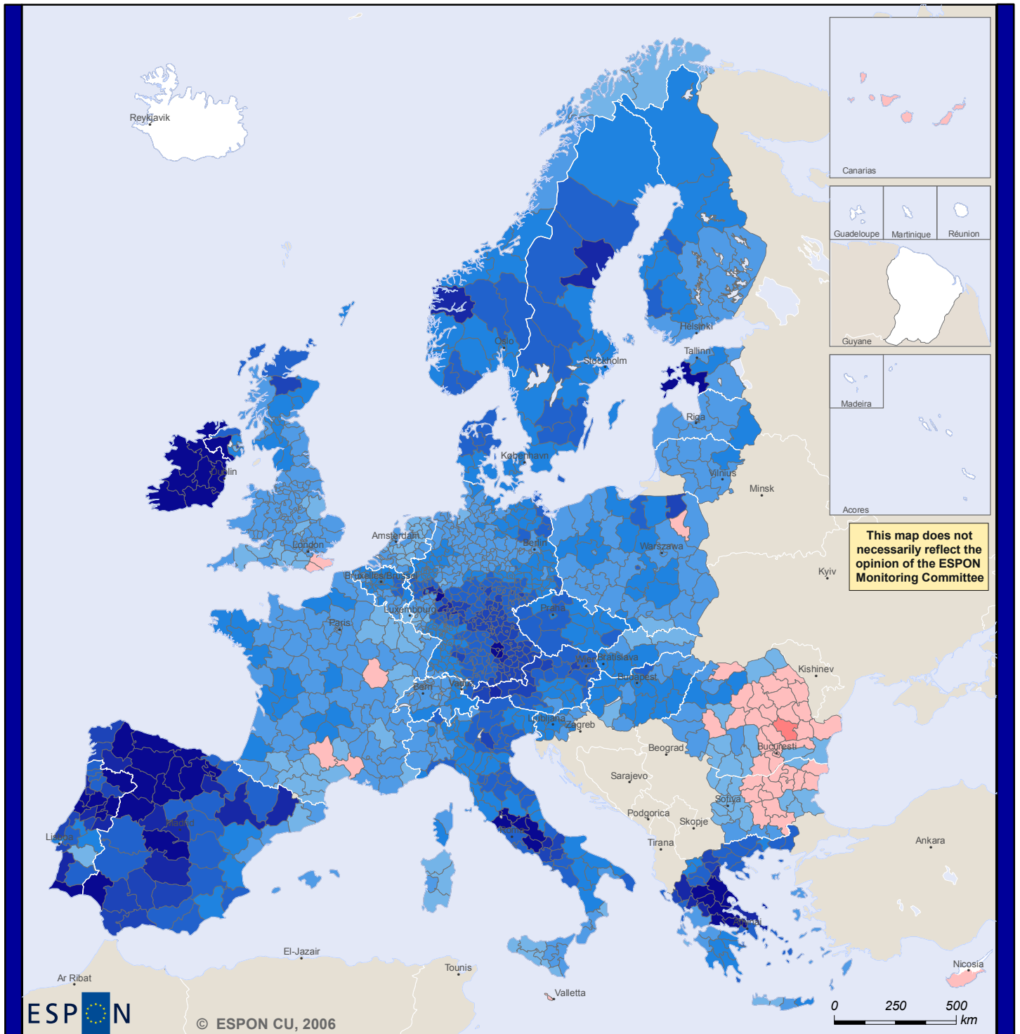
Map 4 Potential accessibility by rail, relative change 2001-2006
