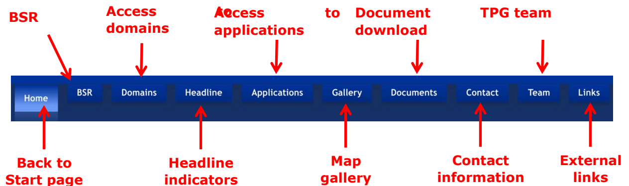
Figure 16 Navigation bar
