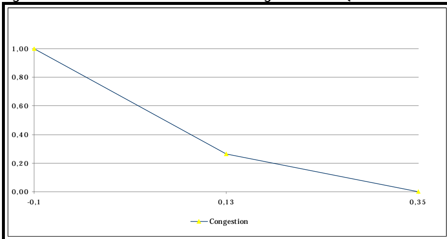
Figure 4.2.4. Value function for criterion Congestion costs (TEQUILA2 – Transport policies)
