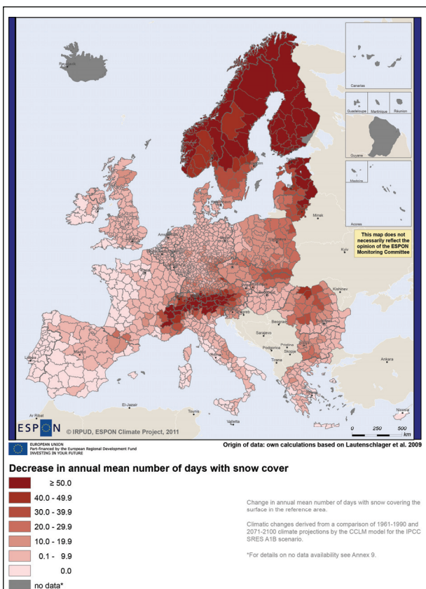
Map 4: Change in annual mean number of days with snow cover
