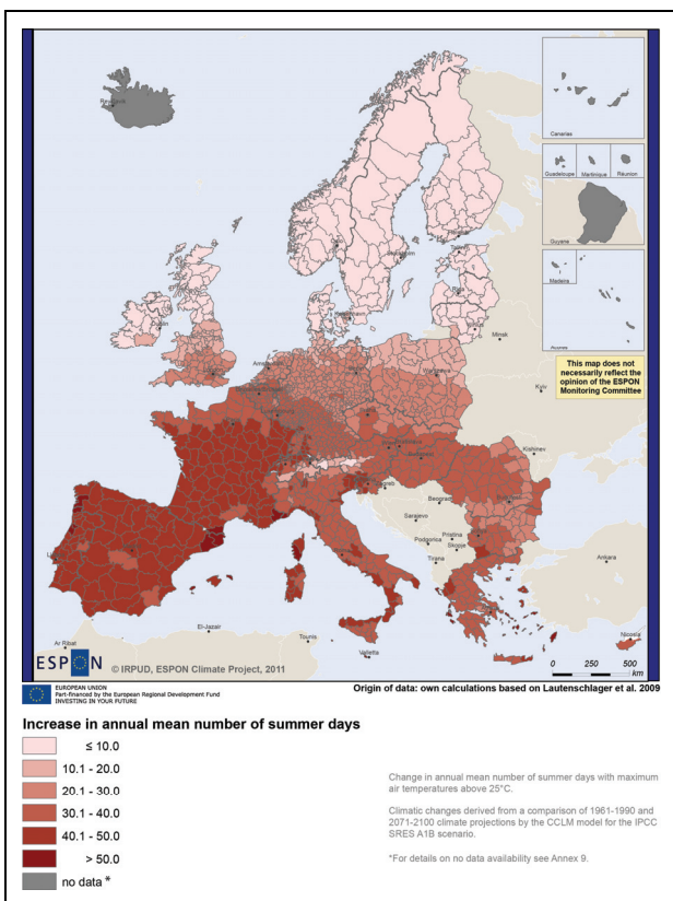
Map 2: Change in annual mean number of summer days
