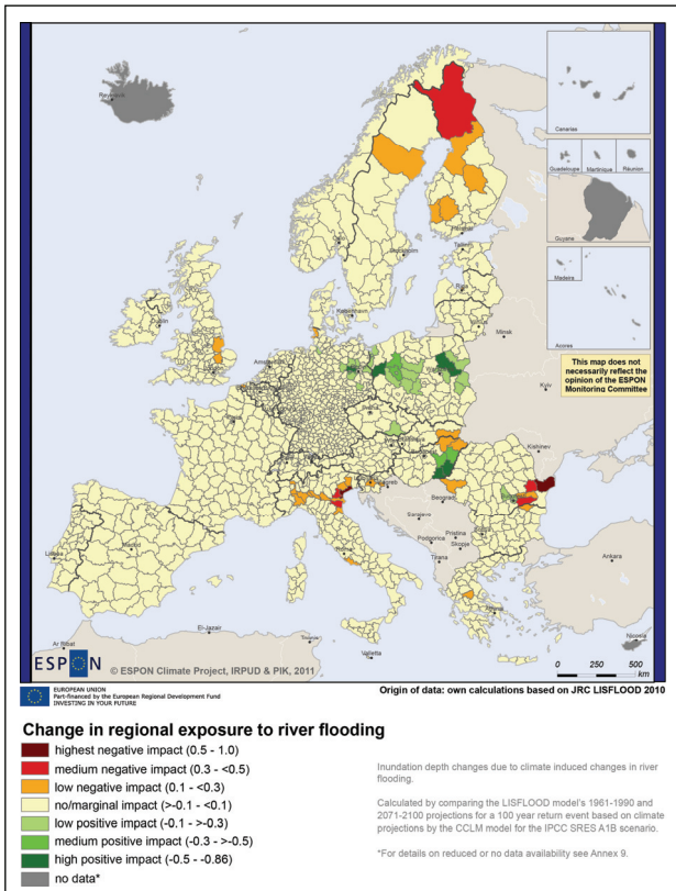
Map 5: Change in regional exposure to river flooding
