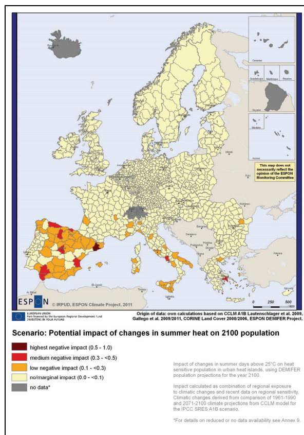
Map 21: Impact of summer heat on 2100 population
