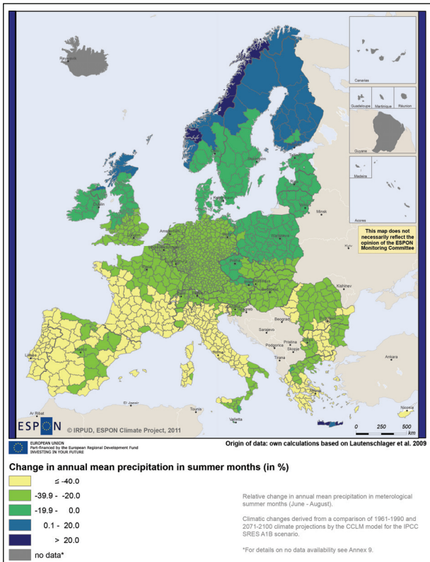
Map 3: Relative change in annual mean precipitation in summer months
