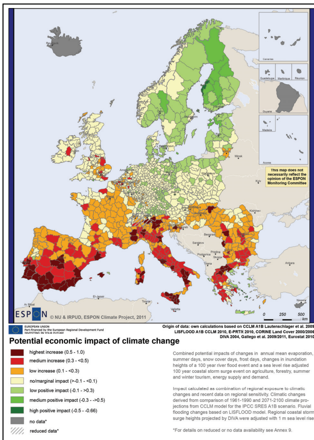
Map 15: Potential economic impact
