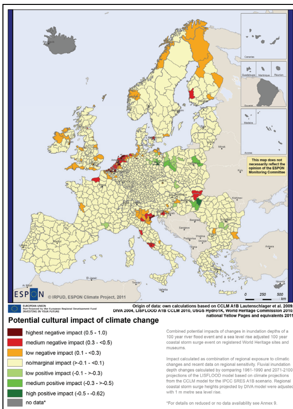
Map 17: Potential cultural impact
