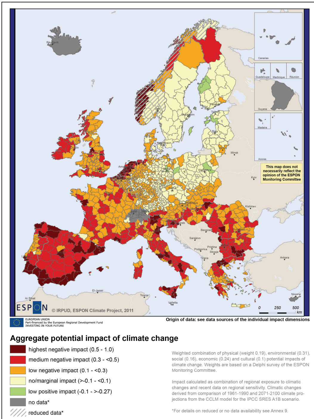
Map 18: Aggregate potential impact of climate change
