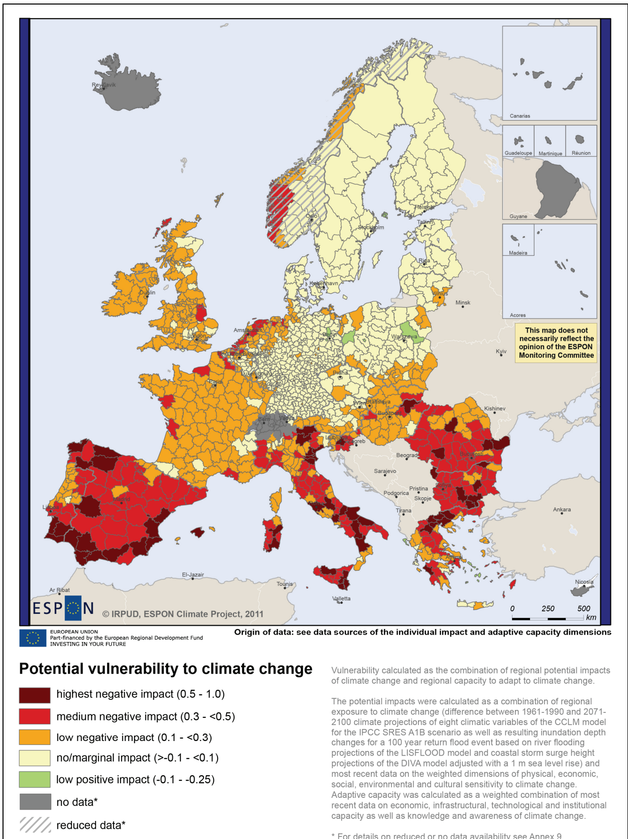
Map 20: Potential vulnerability of European regions to climate change
