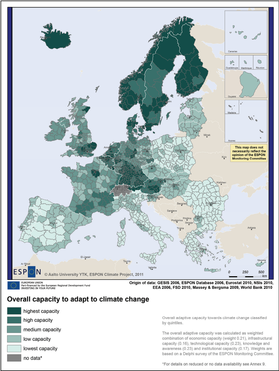
Map 19: Adaptive capacity of European regions in regard to climate change
