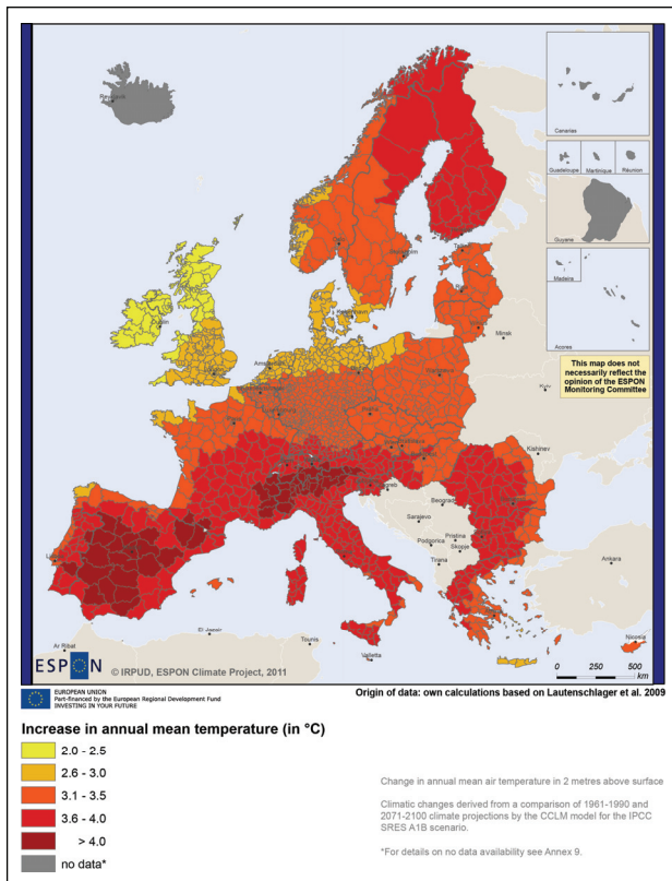
Map 1: Change in annual mean temperature
