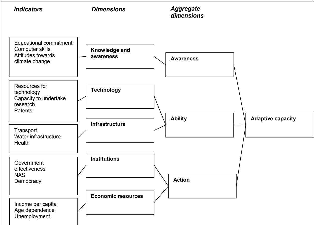
Figure 3: Indicators, dimensions and aggregate dimensions of adaptive capacity
