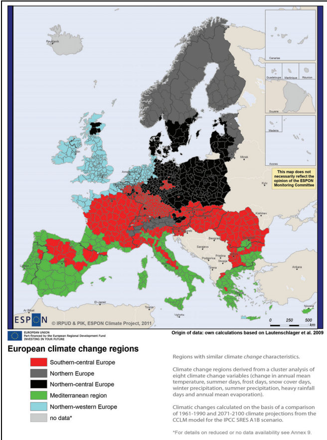
Map 7: Climate change typology
