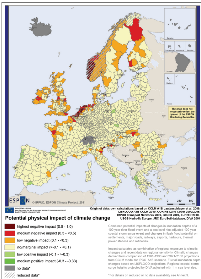
Map 13: Potential physical impact
