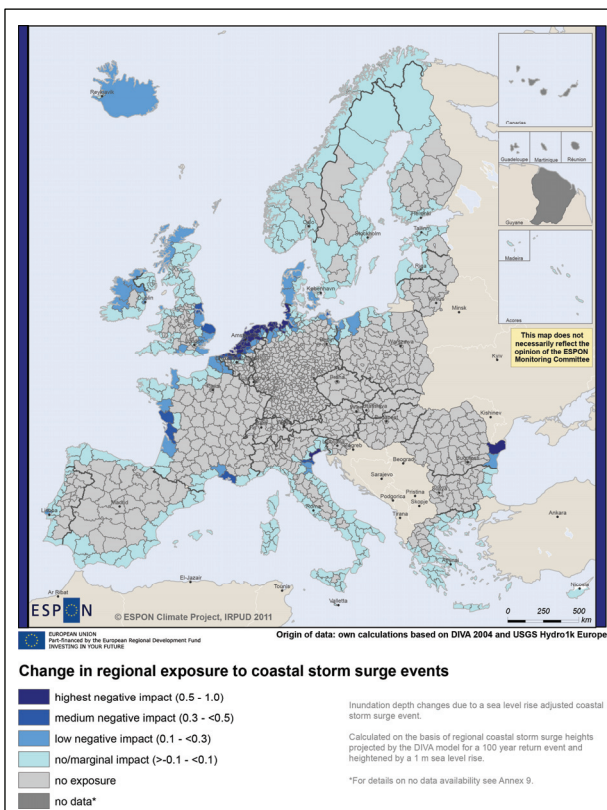
Map 6: Change in exposure to coastal flooding
