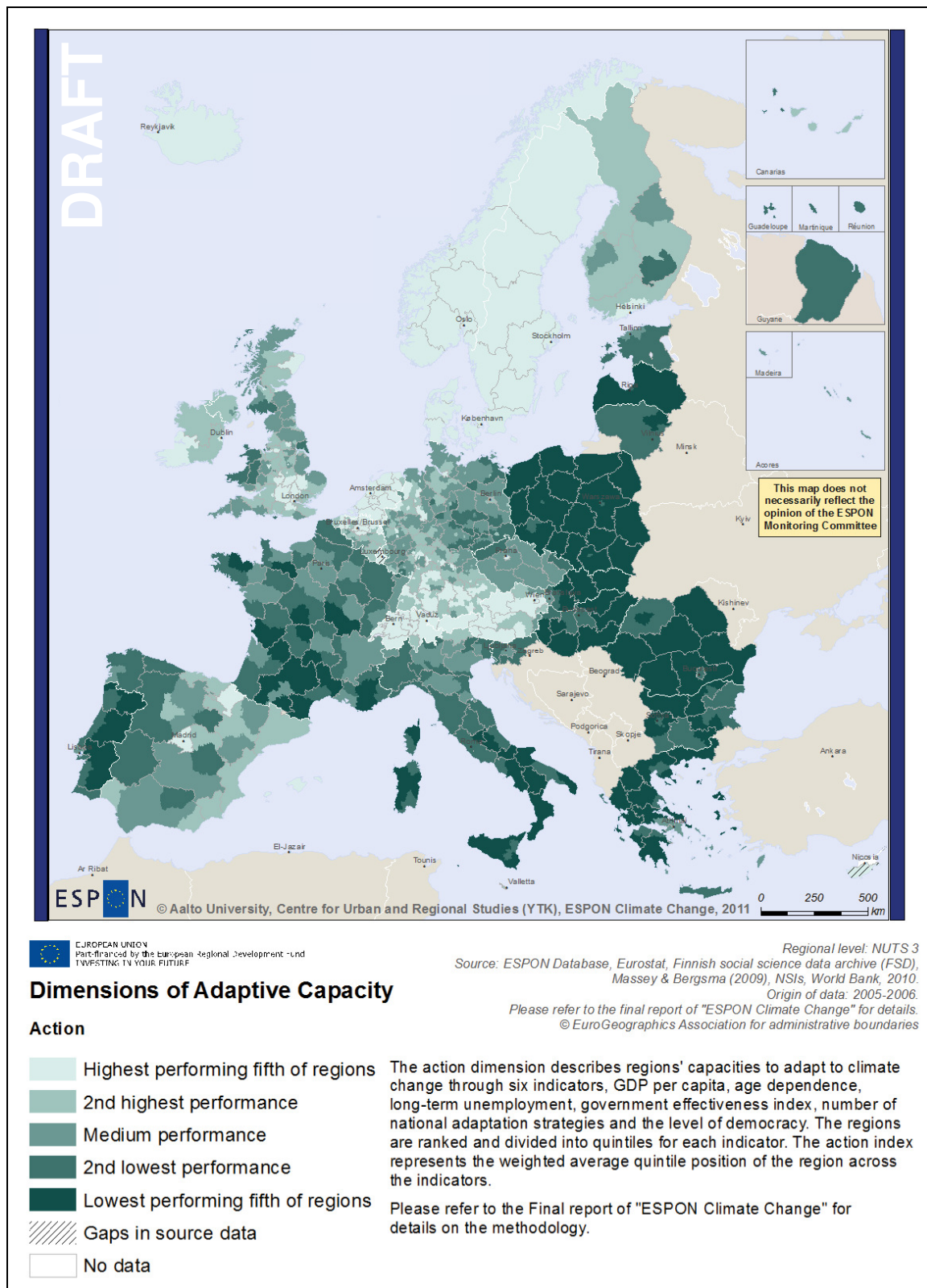
Figure 60: Dimensions of adaptive capacity: Action
