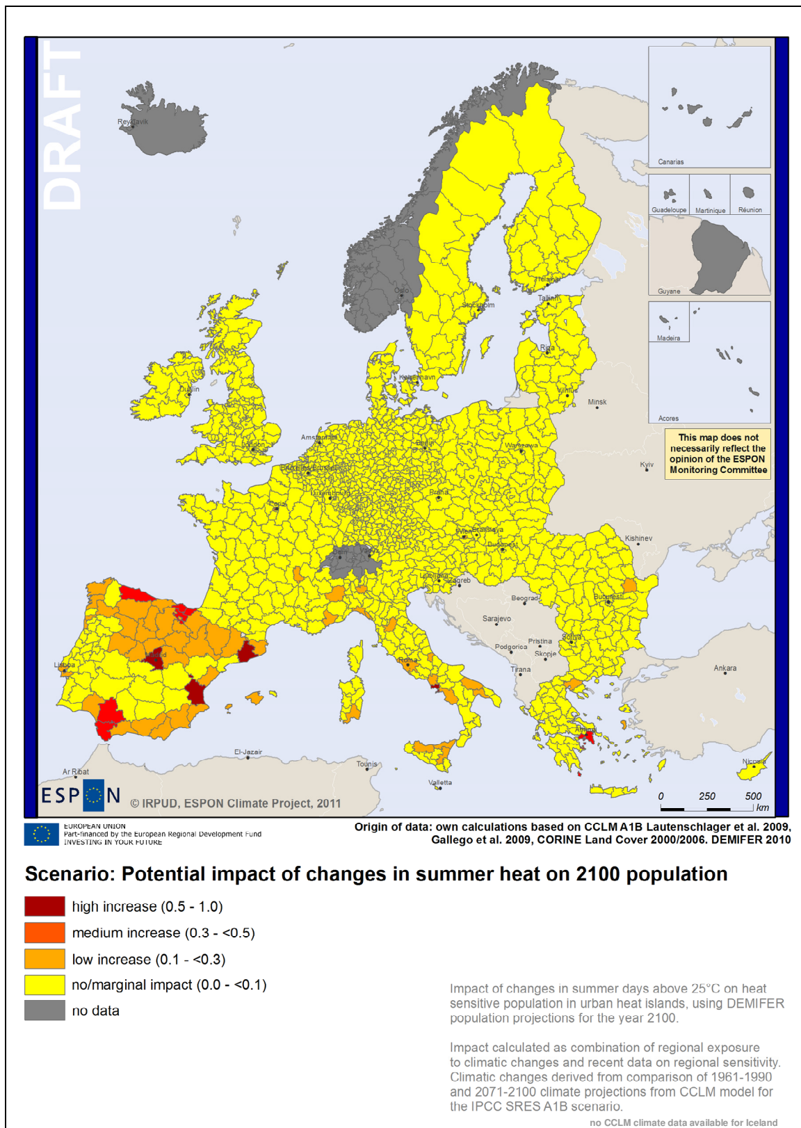
Figure 71: Alternative scenario for impact of summer heat on 2100 population
