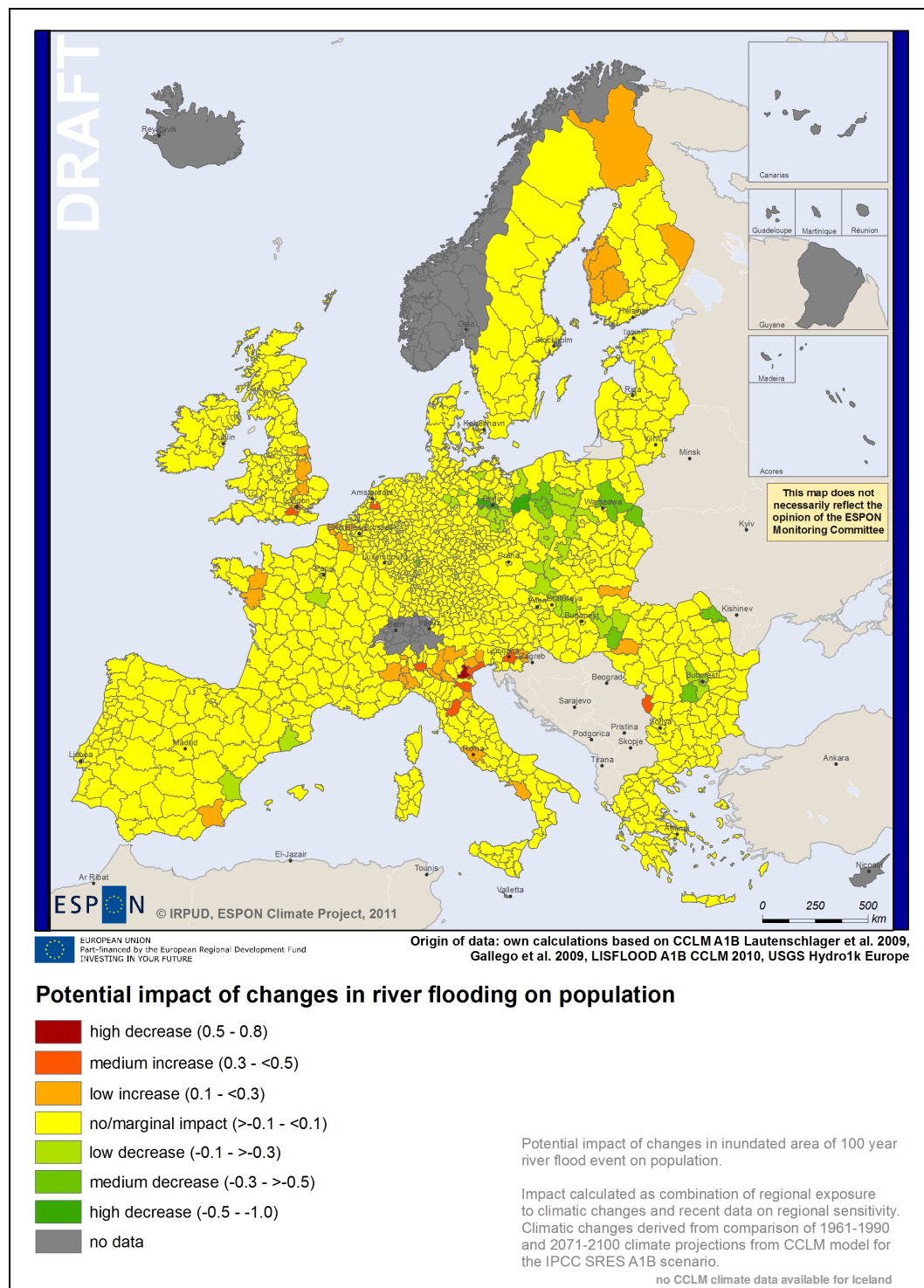
Figure 35: Potential impact of changes in river flooding on population
