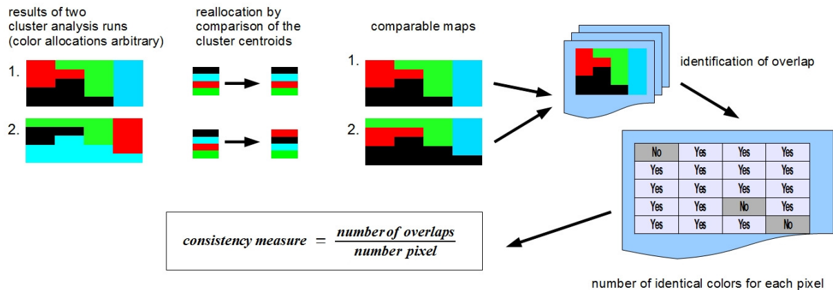
Figure 19: Determination of the number of cluster by means of measuring their consistency (Sietz, in review)
