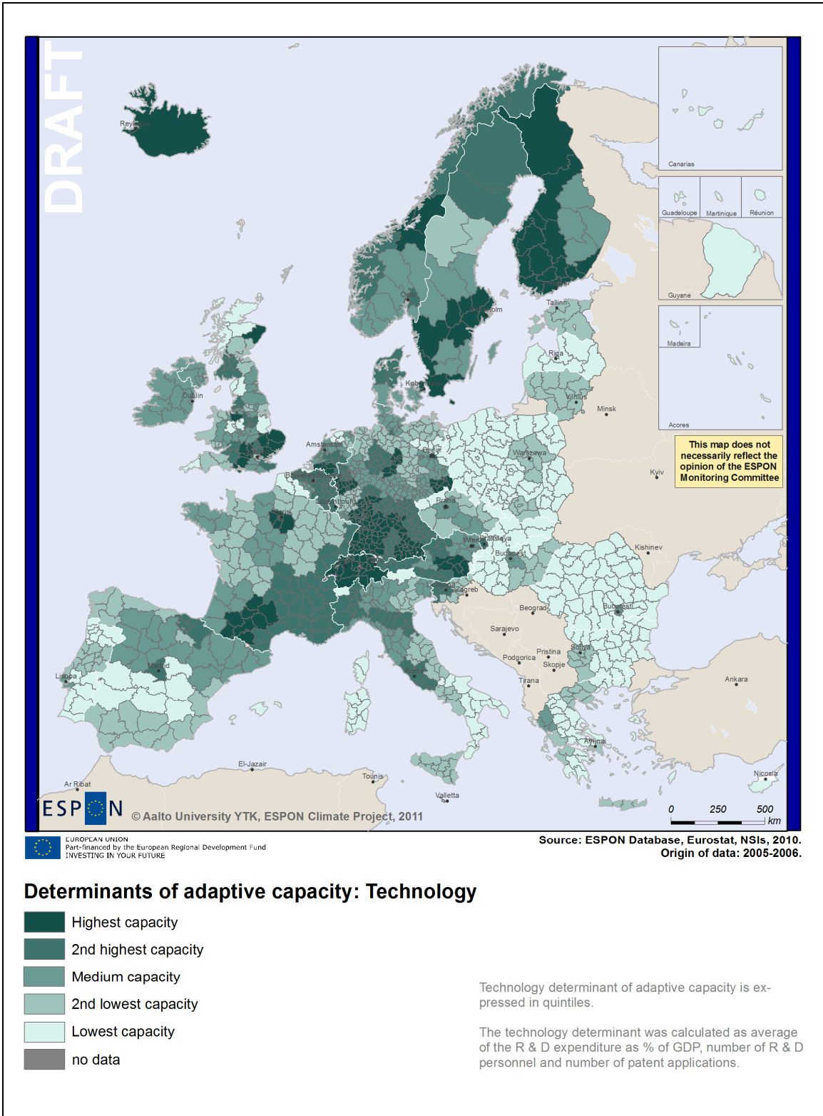
Figure 55: Determinants of adaptive capacity: Technology
