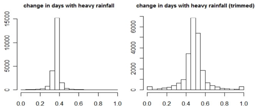
Figure 17: Standardised distributions of the changes in days with heavy rainfall without trimming (left) and with trimming (right).
