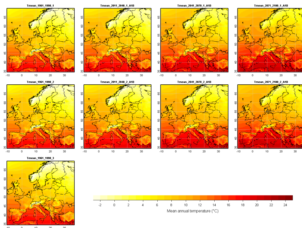
Figure 4: CCLM output on mean annual temperature ( T_{2M\_AV} ), averaged for different timeframes (1961-1990, 2011-2040, 2041-2070, 2071-2100), for different model runs and scenario A1B. (source: Lautenschlager et al. 2009, preparation by PIK)
