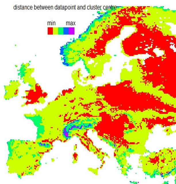
Figure 22: Spatial distribution of the distance of the properties of each data point to the corresponding cluster centre for 5 clusters.
