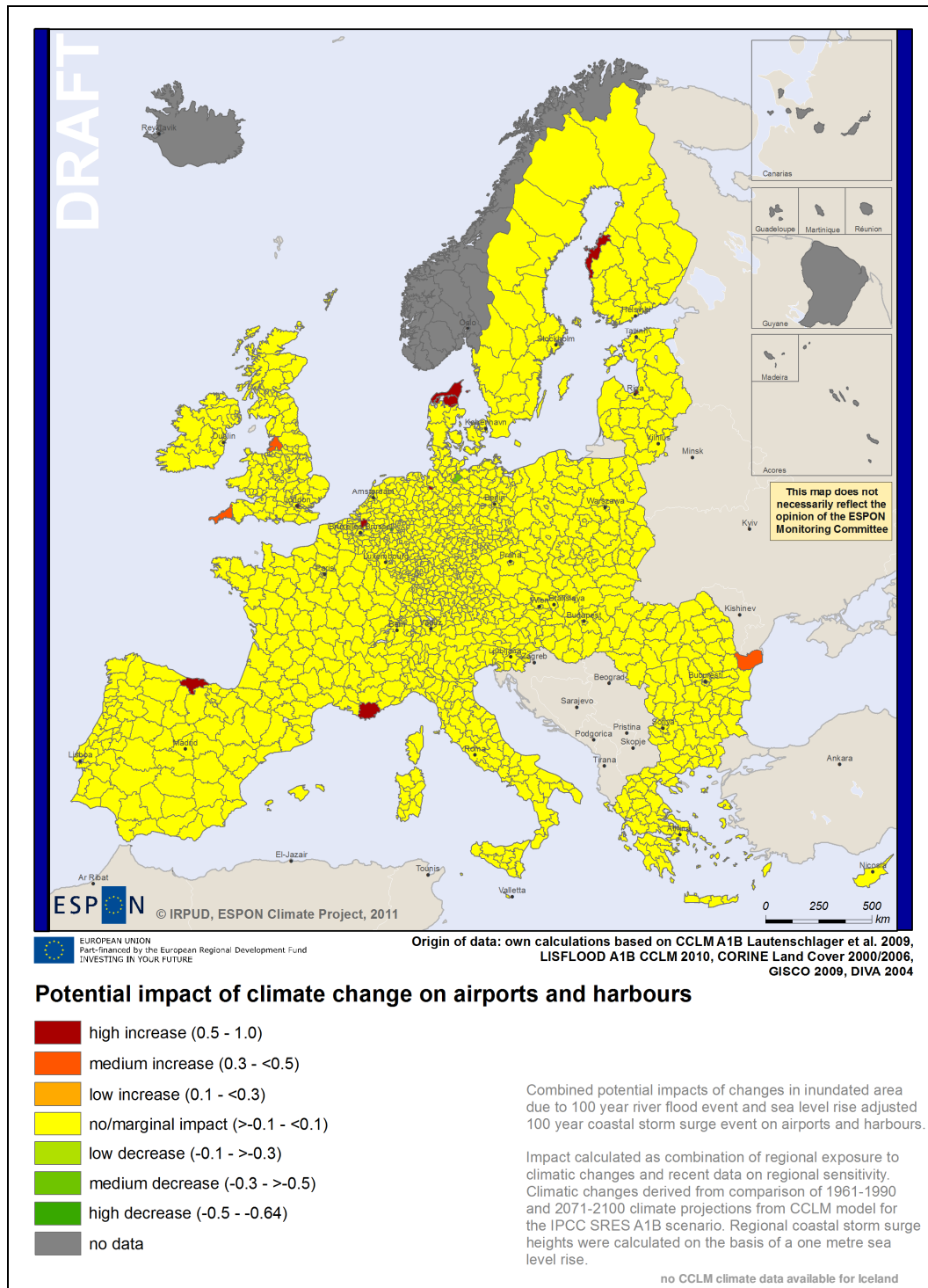
Figure 32: Potential impact of climate change on airports and harbours
