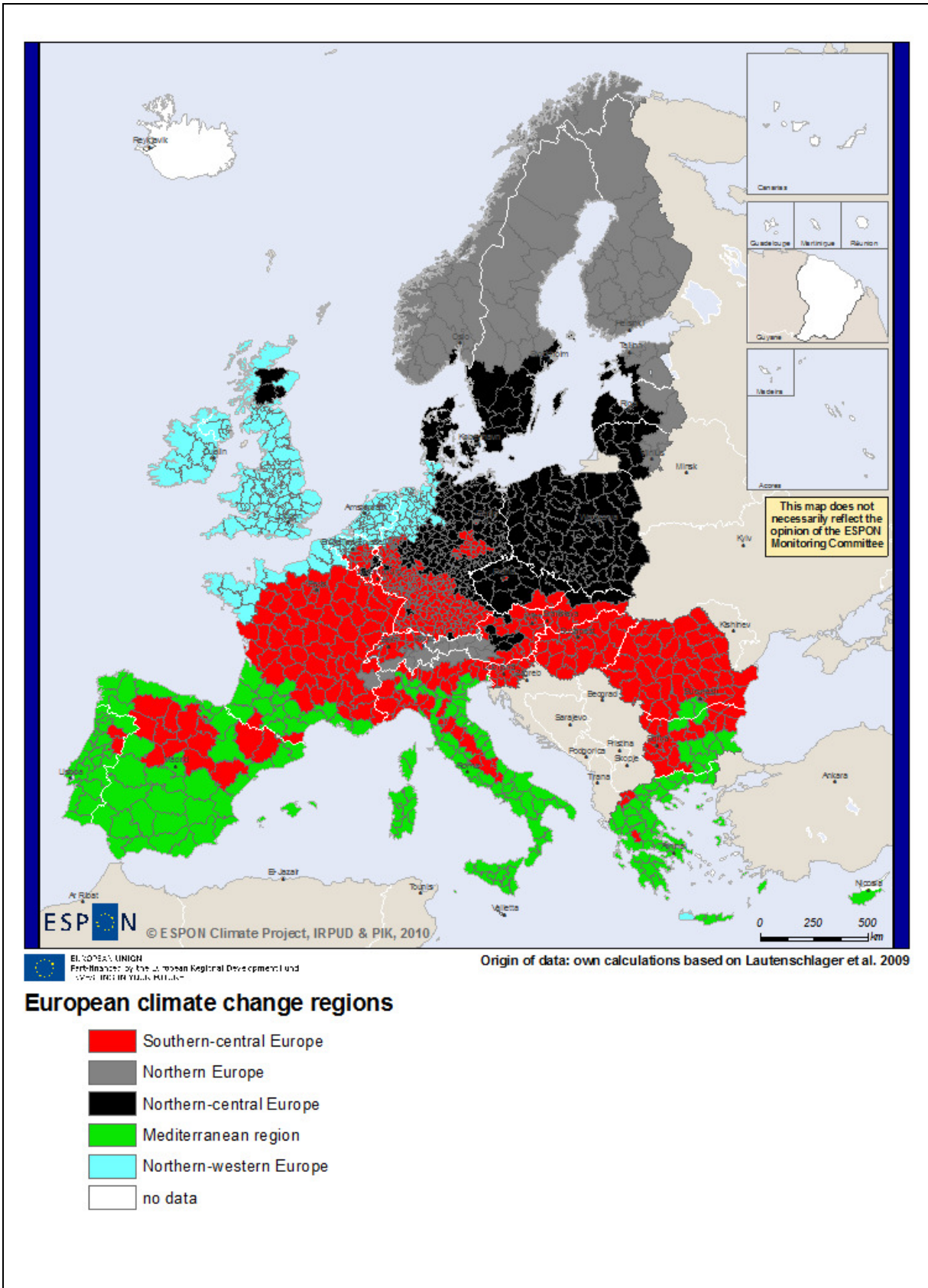
Figure 23: Map of European climate change regions
