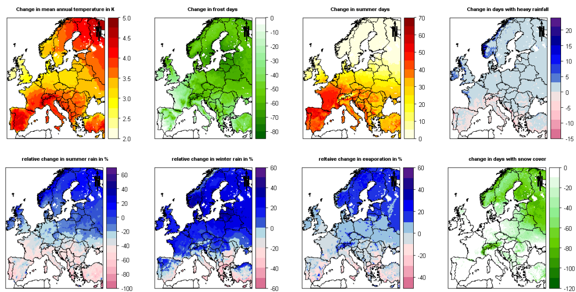
Figure 15: Changes of the eight considered climate variables of the model CCLM between the time periods 1961-1990 to 2071-2100 (Africa is marked with white cells).
