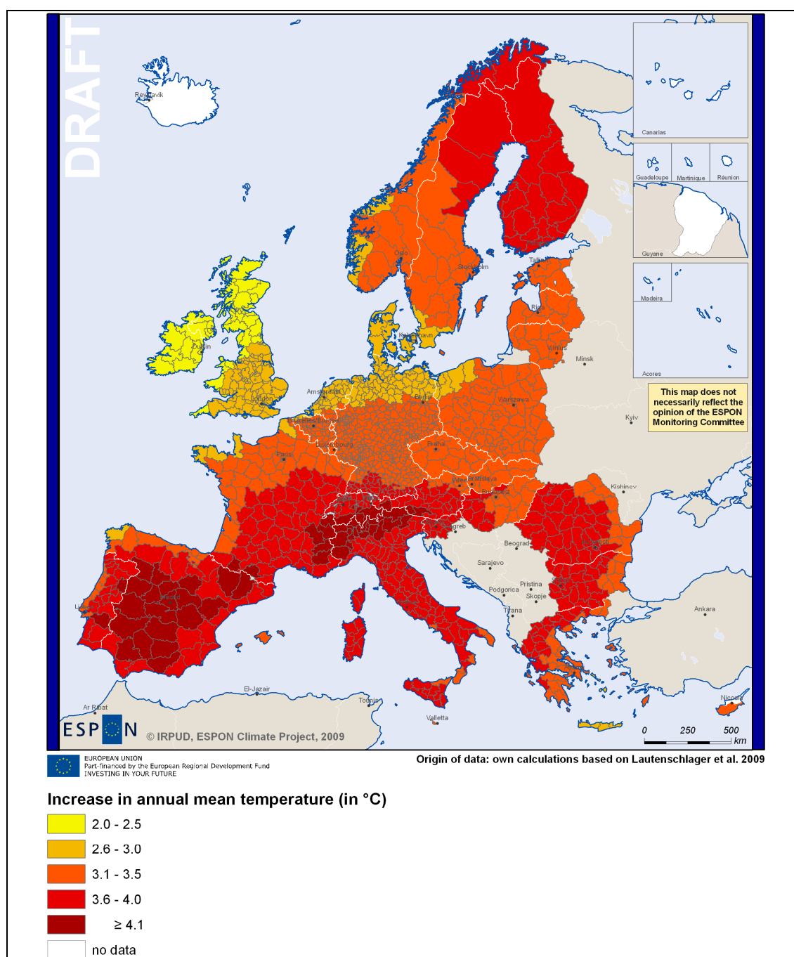
Figure 5: Change in annual mean temperature (EXP_TMEAN)
