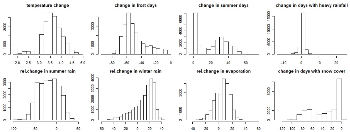
Figure 16: Frequency distribution of the climate variables for the considered cells ( n=22771 )
