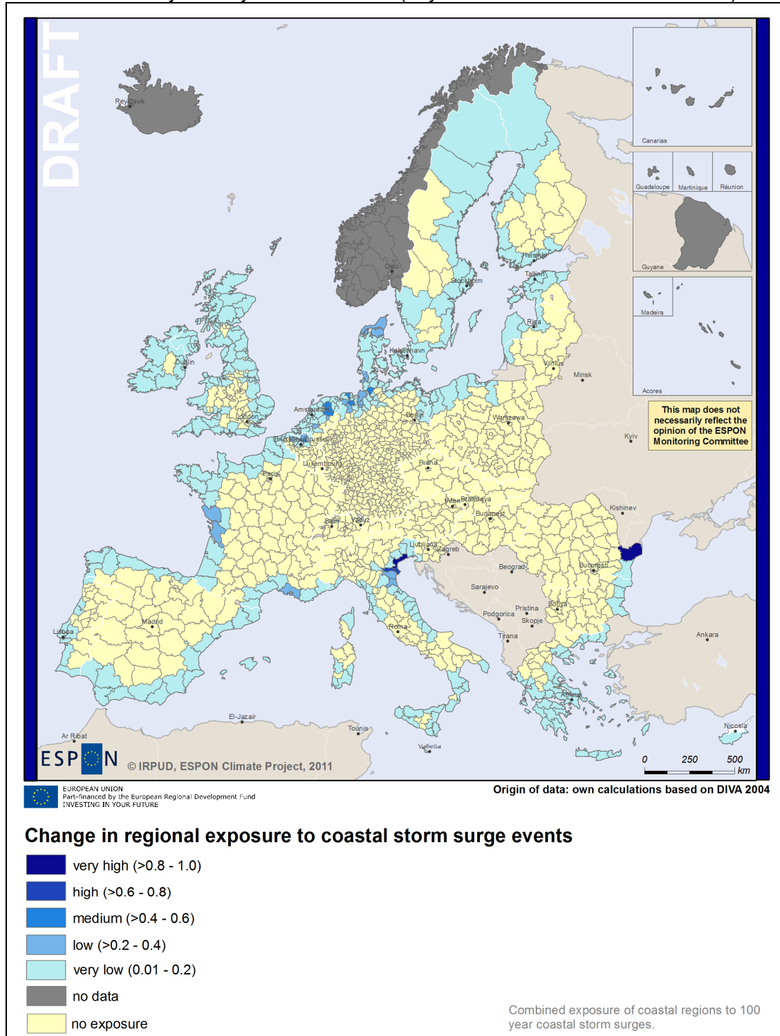
Figure 13: Change in regional exposure to coastal flooding
