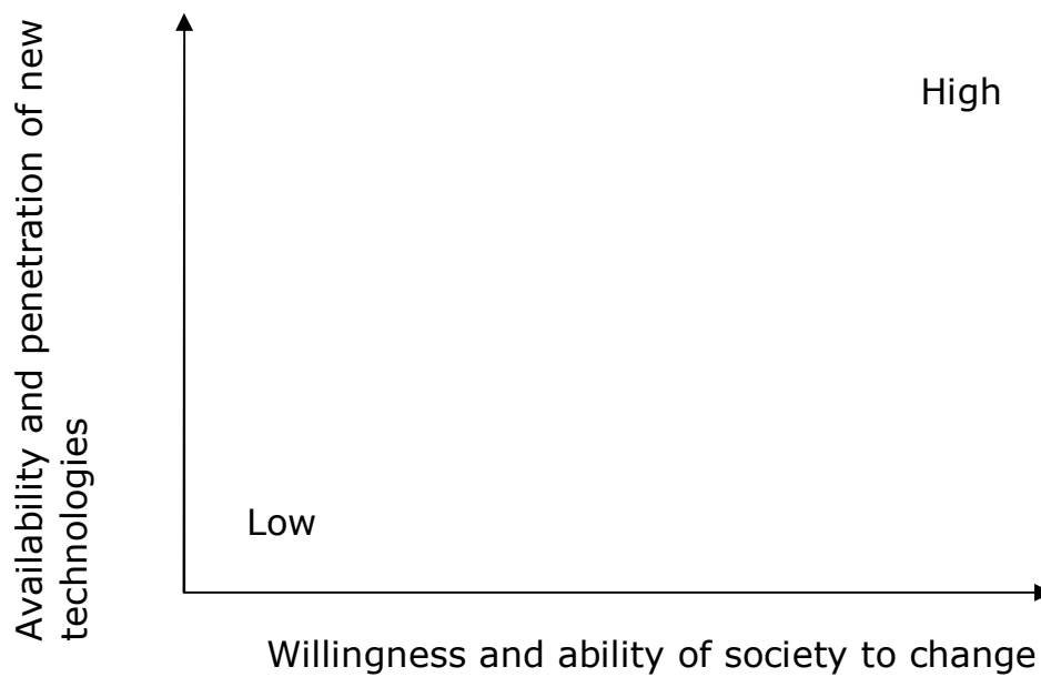
Figure 67: Response space (Tompkins, Adger 2005)
