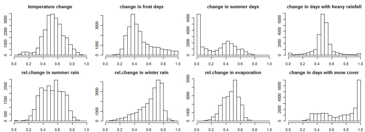
Figure 18: Standardised distributions of the climate variables for the considered cells (n=2277), trimmed values of changes in days with heavy rainfall
