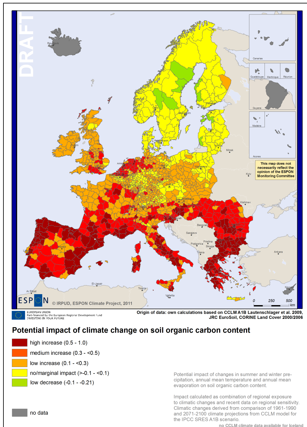
Figure 49: Potential impact of climate change on soil organic carbon content
