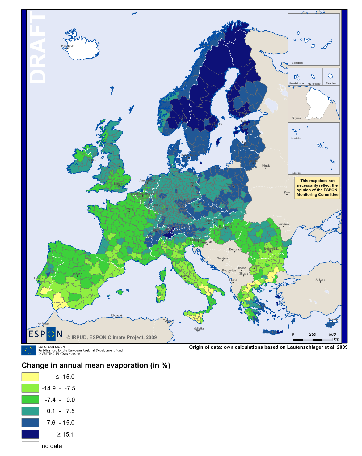
Figure 11: Relative change in annual mean evaporation (EXP_EVAP)
