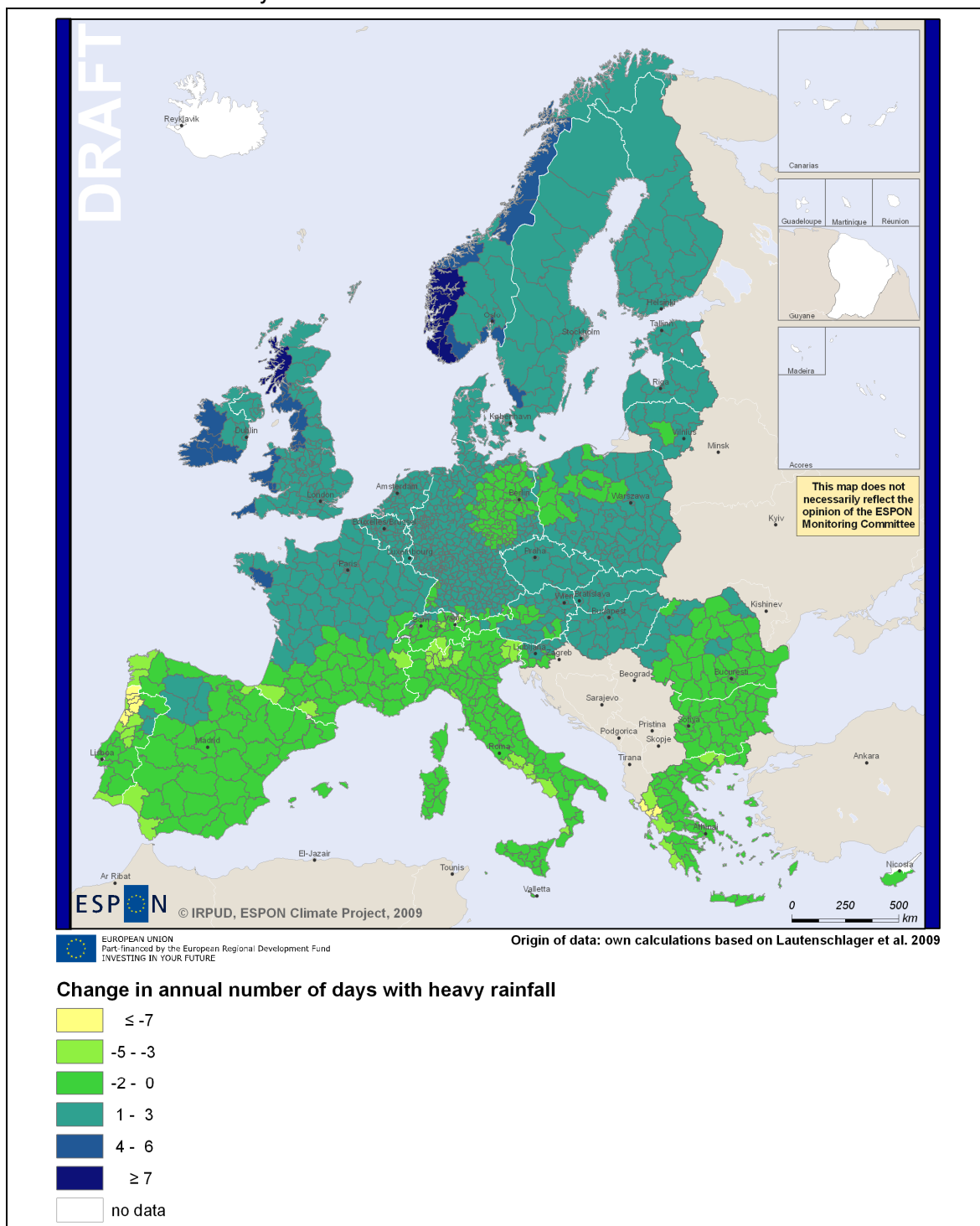
Figure 10: Change in annual mean number of days with heavy rainfall (EXP_HR)
