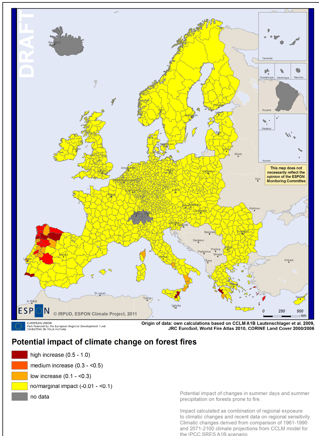
Figure 46: Potential impact of climate change on forest fires
