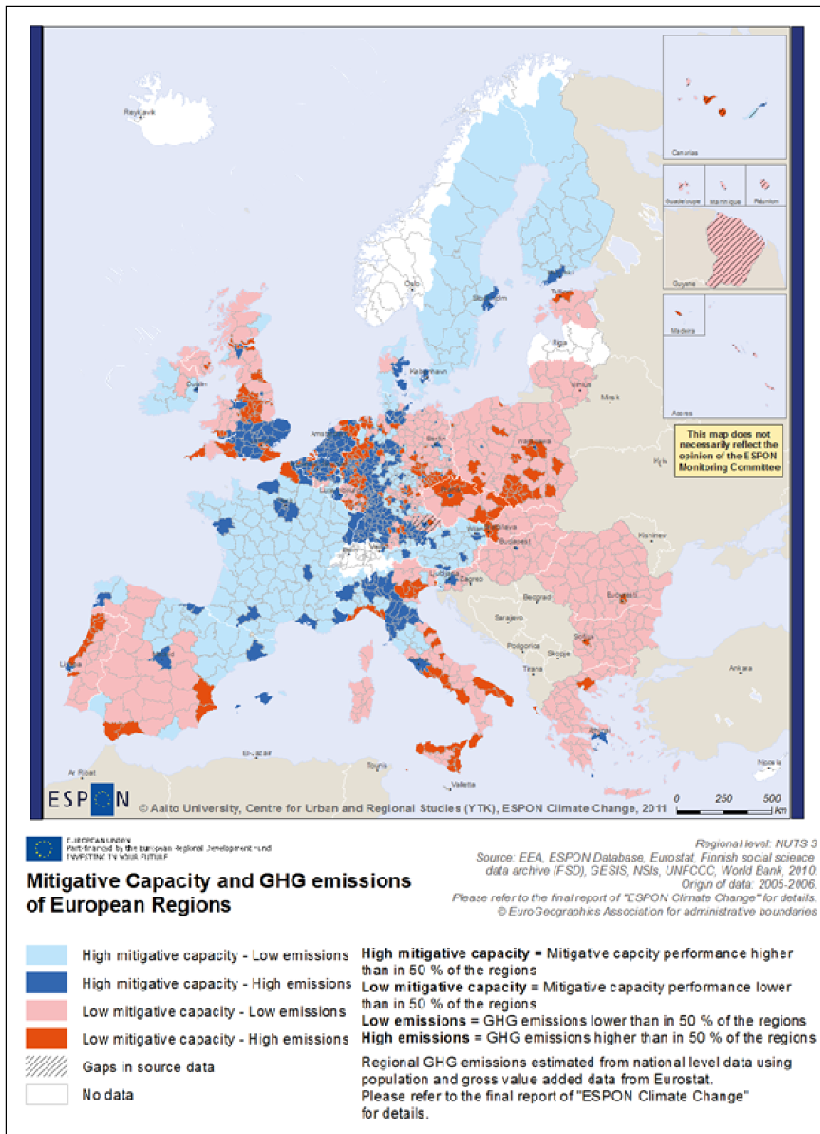
Figure 66: Mitigative capacity and GHG emissions of European regions.
