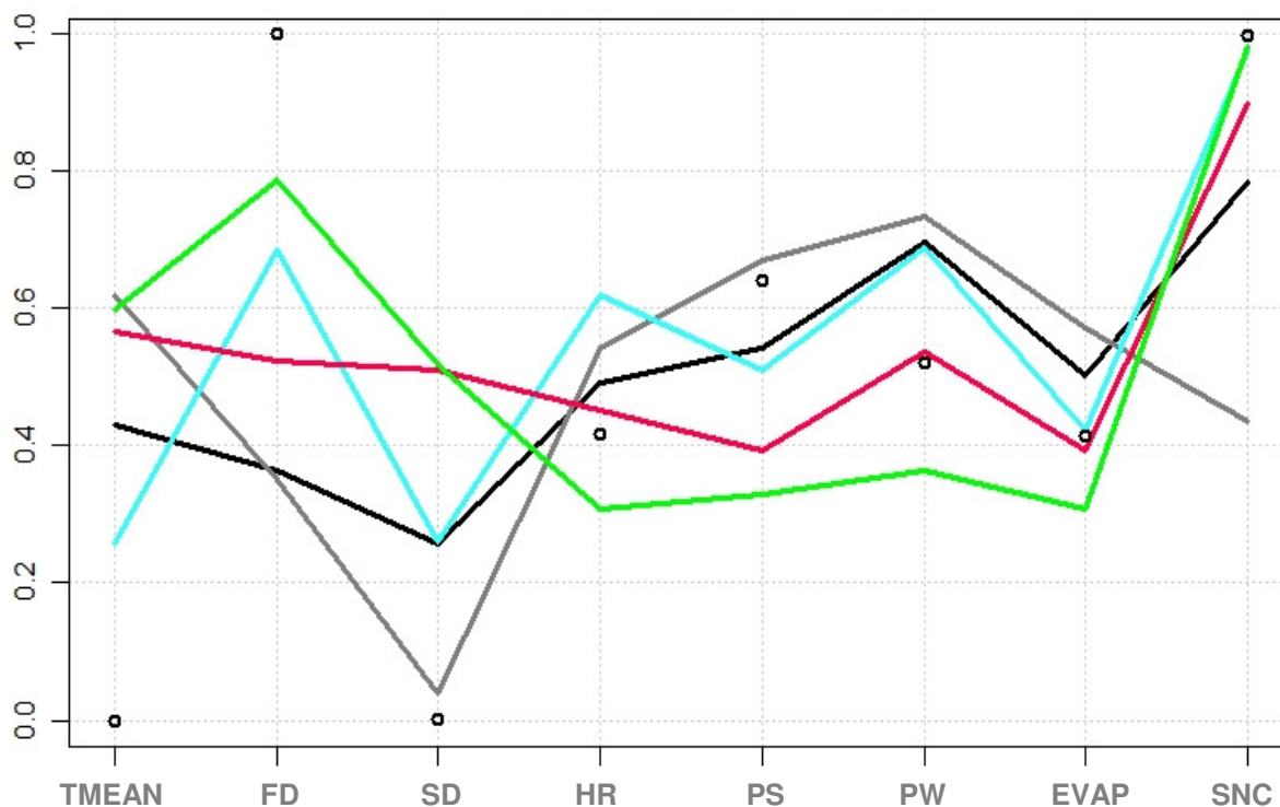
Figure 21: Cluster feature graph for detailed information about the cluster characteristics for the eight climate variables (mean values). Additionally the black circles show the location of the value of zero.
