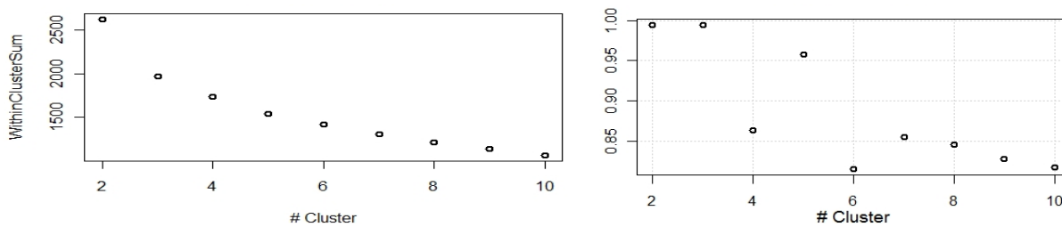
Figure 20: Comparison of the traditional elbow-criterion (left) and the consistency measure (right)
